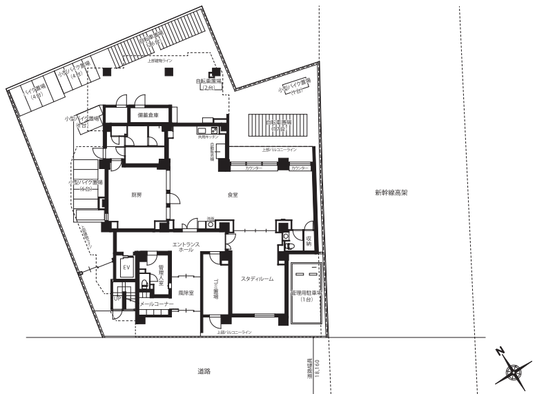
1F
