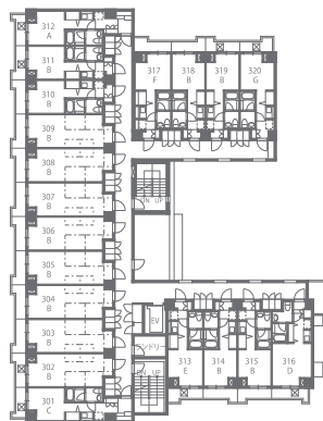
[3F 平面図]
