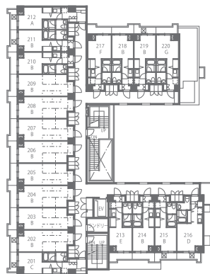
[2F 平面図]
