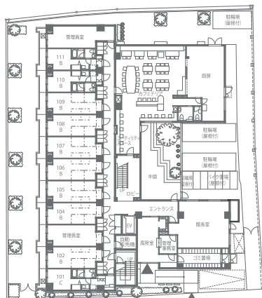
[1F 平面図]
